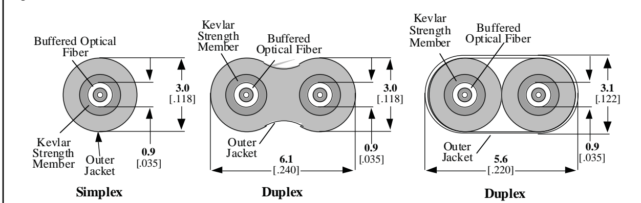
Figure 2-13—Indoor Cables
